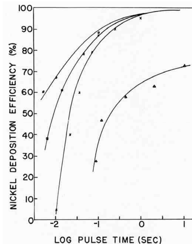
Figure 6 - Nickel deposition efficiency vs. pulse time. \Delta = 5 \text{ mA/cm}^2 , \times = 10 \text{ mA/cm}^2 ; \square = 50 \text{ mA/cm}^2 ; \circ = 100 \text{ mA/cm}^2 .
