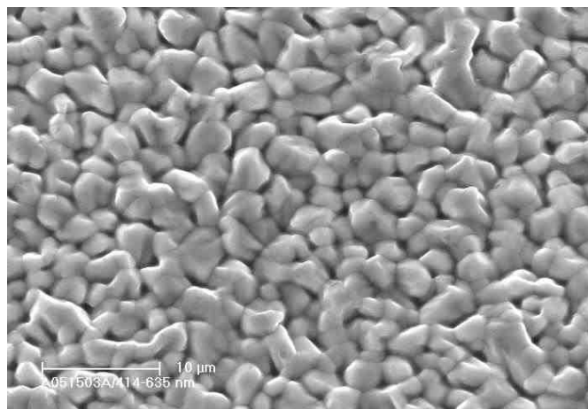
Figure 8 - SEM image of the surface of the Sn-Zn deposit after a potentiostatic scan from the OCP to -800 \text{ mV}_{\text{SCE}} in the 0.1M \text{Na}_2\text{SO}_4 (pH 3.6) corrosive solution. From Maurer, et al. 69
