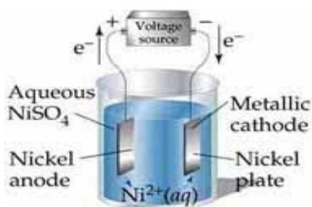
Fig. 1 Simple Nickel Plating Cell
