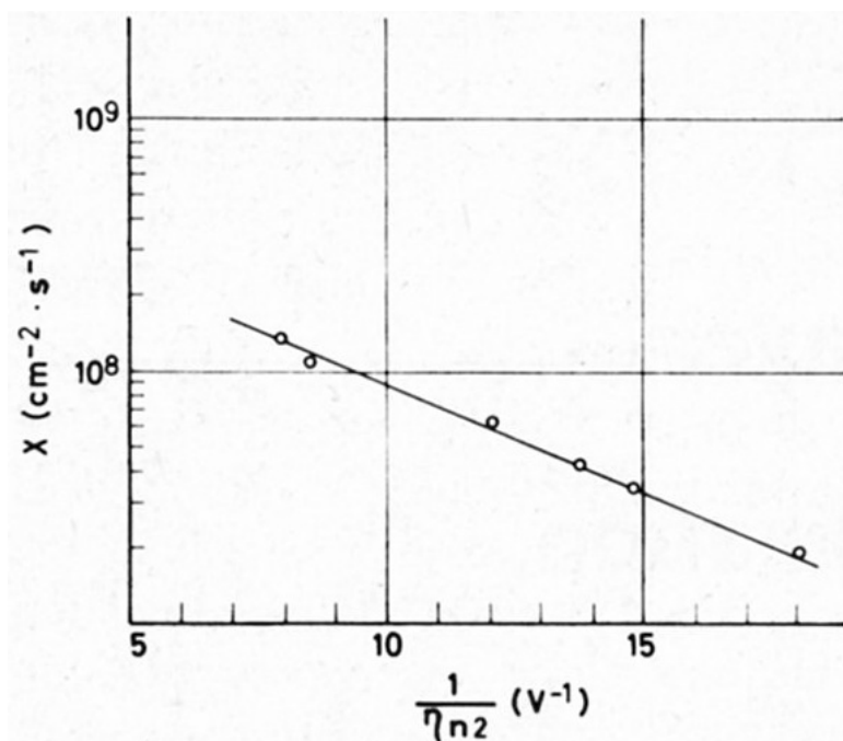
Figure 1 - Rate of the formation of growth layers ( \log X ) vs the reciprocal overpotential of nucleation (deposition of copper in presence of o-phenanthroline).
