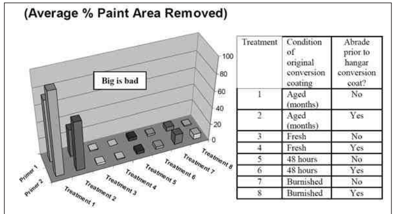
Figure 2—The adhesion of primers based on the surface treatment following the rivet manufacturing processes.
