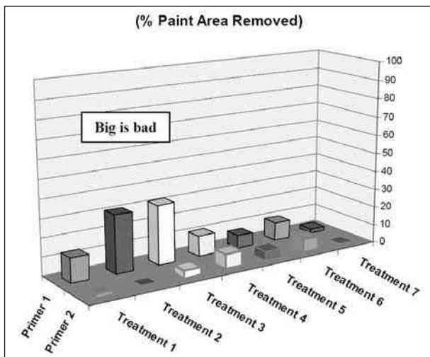
Figure 7—The effect of the rivet new sol-gel finish as painted in production.
