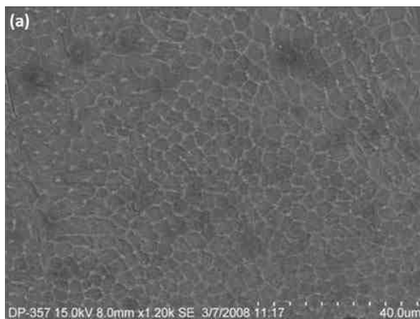
Figure 4— (a) SEM micrograph (etched with 1:1:1::HCl:HNO 3 :H 2 O) and (b) EDS spectra on 316 stainless steel coatings processed by 500 W fiber laser with a powder mass flow rate of 0.068 g/sec and a traverse speed of 5 mm/sec.
