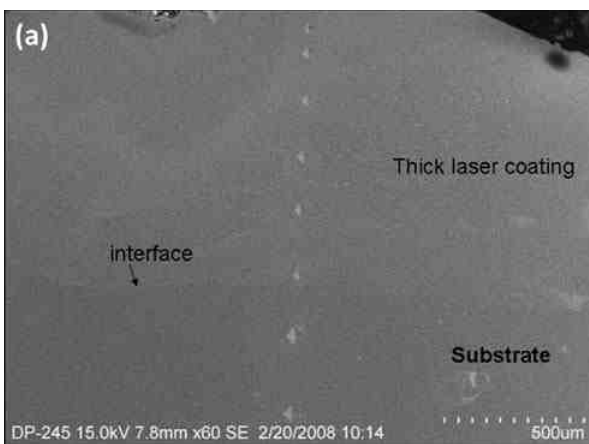
Figure 2—SEM micrographs of (a) the cross-section of a thick laser coating on 1018 steel, showing micro-indentation marks and (b) an enlarged view of the interfacial region, deposited by fiber laser at 800 W with a powder mass flow rate of 0.068 g/sec and a traverse speed of 5 mm/sec.
