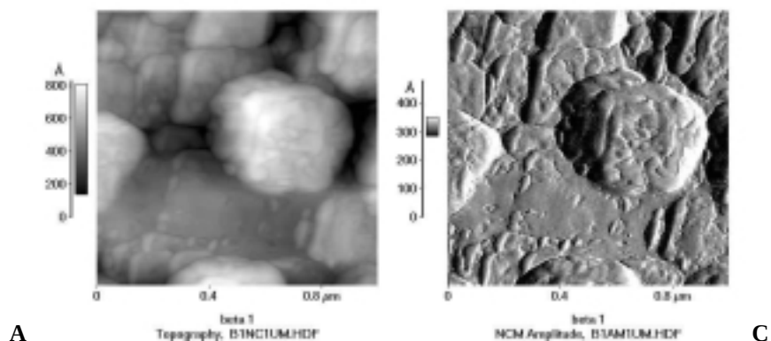
Figure 8: AFM images of copper thin film from bath N; 30°C, 20 mA/cm 2 , 30s, no stirring onto Si/SiO 2 /TiN/Cu 0.1 μm (A: contact mode; B: lateral force mode; C: non contact mode).
