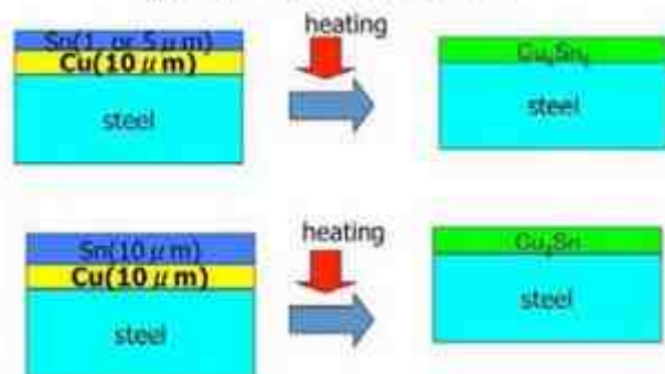
Figure 6 - Schematic illustration for producing a tin-copper alloy film by HSSL. 26
