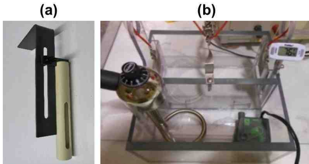
Figure 3 - (a) In-site 1 cell; (b) test cell with accessories.
