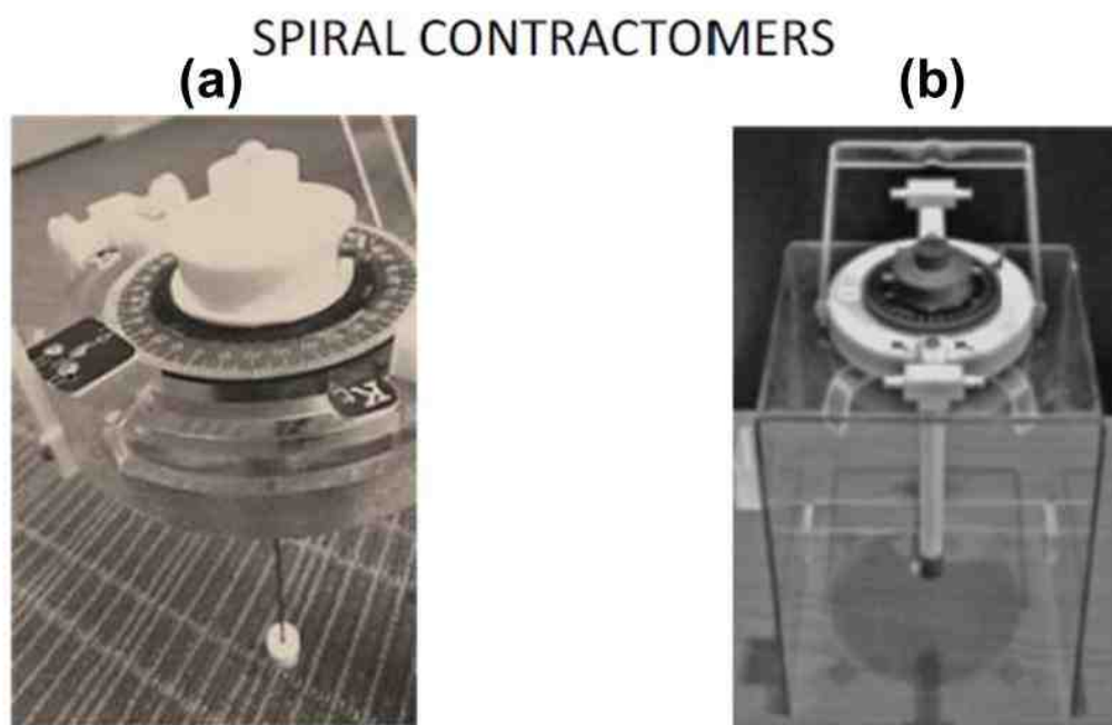
Figure 1 - Spiral contractometer designs: (a) Prior design; (b) New design.
