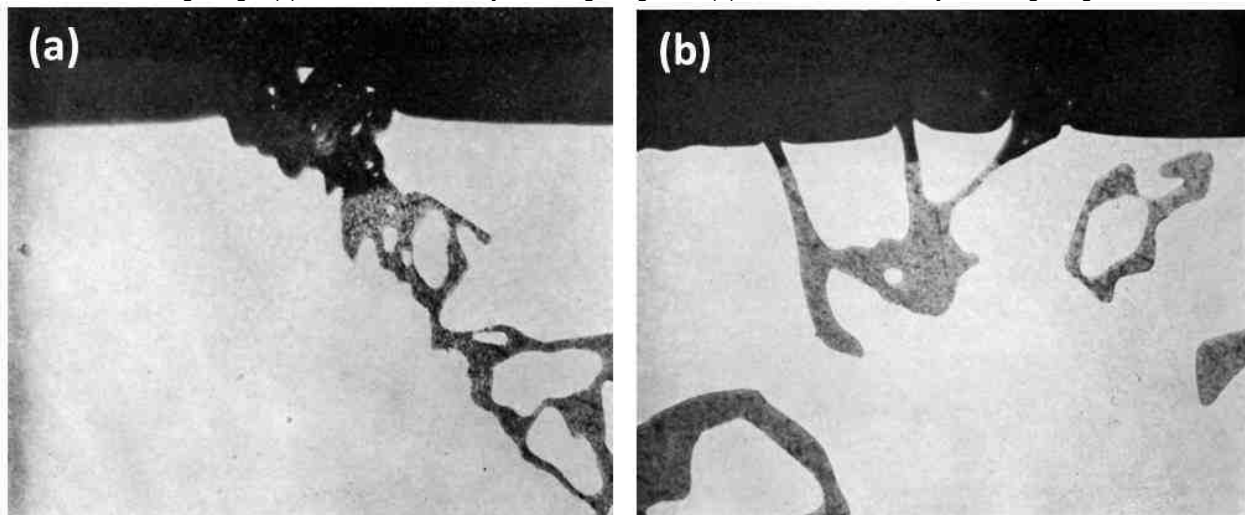
Figure 6 - Cross-section of anodized Al-6.4 Mg-3.7 Si alloy illustrating the behavior of \text{Mg}_2\text{Si} (500 \times ): (a) as cast structure and (b) in homogenized condition.
