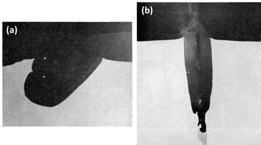
Figure 8 - Cross-section of anodized Al-2Cr alloy showing the behavior of CrAl_3 (1000 \times ): (a) completely dissolved and (b) almost completely dissolved.
