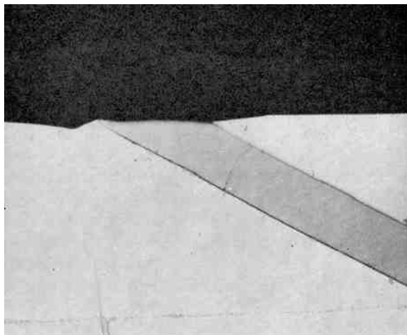
Figure 4 - Cross-section of anodized Al-5Fe alloy showing anodized \text{FeAl}_3 (500 \times ).
