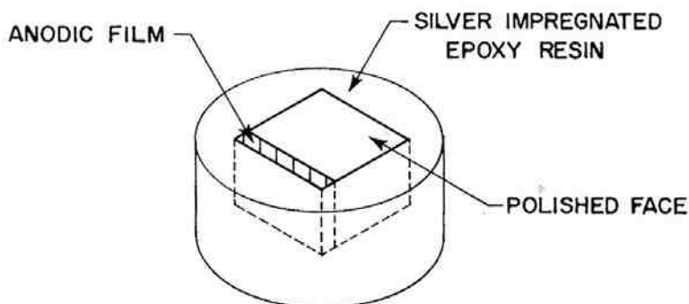
Figure 1 - Specimen for electron probe microanalysis.
