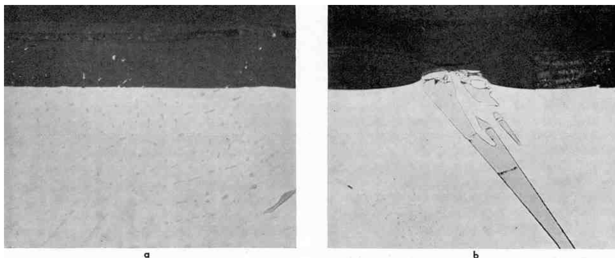
Figure 2 - Cross-section through anodized Al-3Mn alloy: (a) small MnAl 6 particles (1000×); (b) large MnAl 6 particle (500×).
