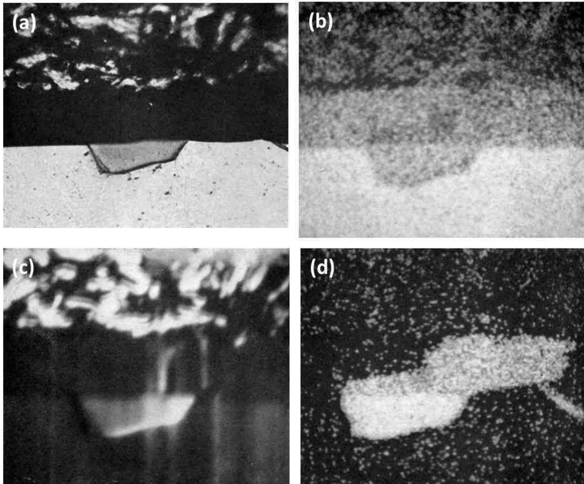
Figure 5 - Cross-section of anodized Al-5Fe alloy showing the behavior of \text{FeAl}_3 (600 \times ): (a) optical micrograph; (b) electron scanning image; (c) Al K \alpha radiation x-ray scanning image and (d) Fe K \alpha radiation x-ray scanning image.
