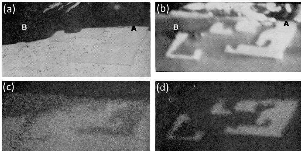
Figure 3 - Cross-section of anodized Al-3Mn alloy showing the behavior of MnAl_6 (800 \times ): (a) optical micrograph; (b) electron scanning image, (c) Al K \alpha radiation x-ray scanning image and (d) Mn K \alpha radiation x-ray scanning image.
