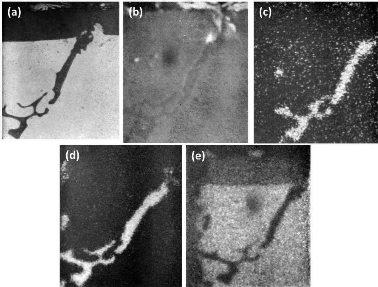
Figure 7 - Cross-section of anodized Al-6.4 Mg-3.7 Si showing the behavior of Mg_2Si (500 \times ): (a) optical micrograph; (b) electron scanning image; (c) Mg K \alpha radiation x-ray scanning image; (d) Si K \alpha radiation x-ray scanning image and (e) Al K \alpha radiation x-ray scanning image.
