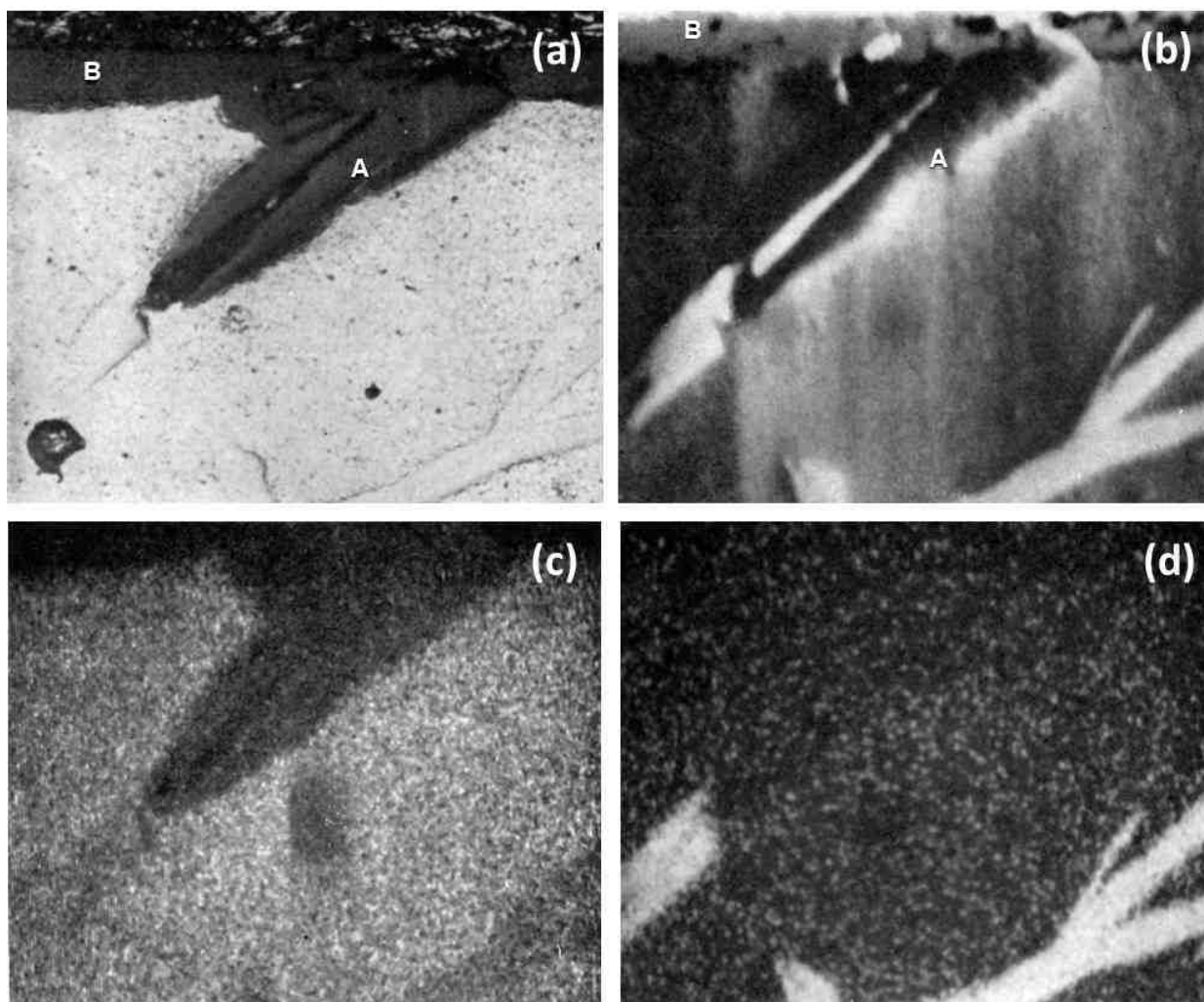
Figure 9 - Cross-section of anodized Al-Cr alloy showing the behavior of CrAl 7 (450 \times ): (a) optical micrograph, (b) electron scanning image, (c) Al K \alpha radiation x-ray scanning image, (d) Cr K \alpha radiation x-ray scanning image.
